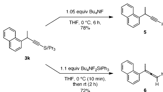
Scheme 3. Desilylation of Hydroalkynylation Product 3k
