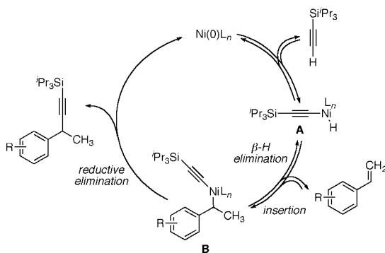
Scheme 2. Plausible Reaction Mechanism of the Hydroalkynylation of Styrenes
