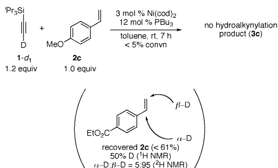
Scheme 1. Reaction of p -Methoxystyrene with Deuterated Triisopropylsilylacetylene 1-d 1
